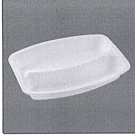
Kebab Two Compartment Container عبوة كebab بقسمين Product Code: 000232 Dimensions (mm): 296 x 225 x 43
